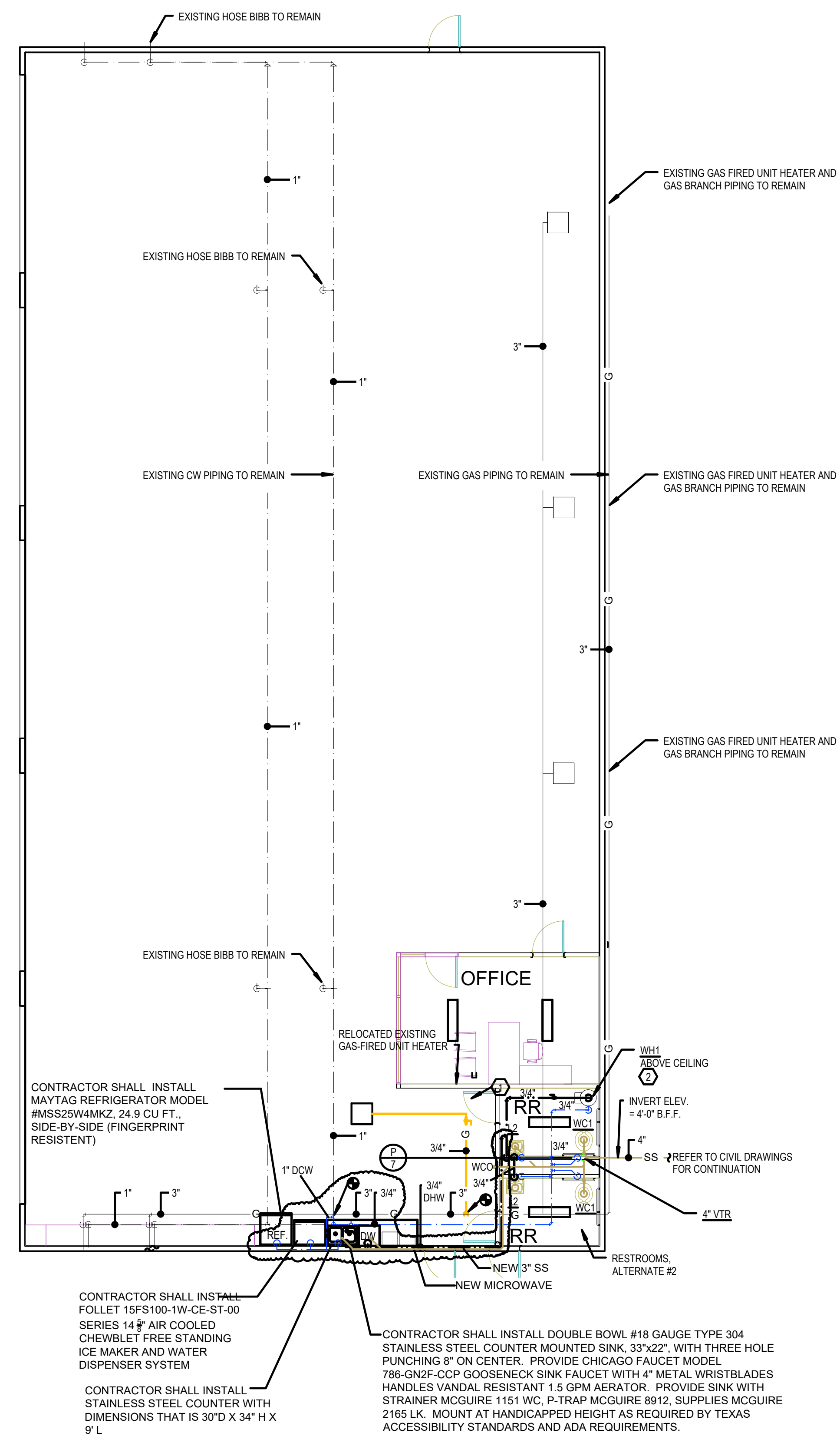
1 MAINTENANCE BUILDING PLAN - PLUMBING 1/8" = 1'-0"
